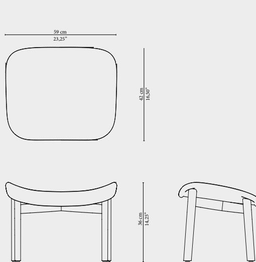
FOOTREST 02590-XX
